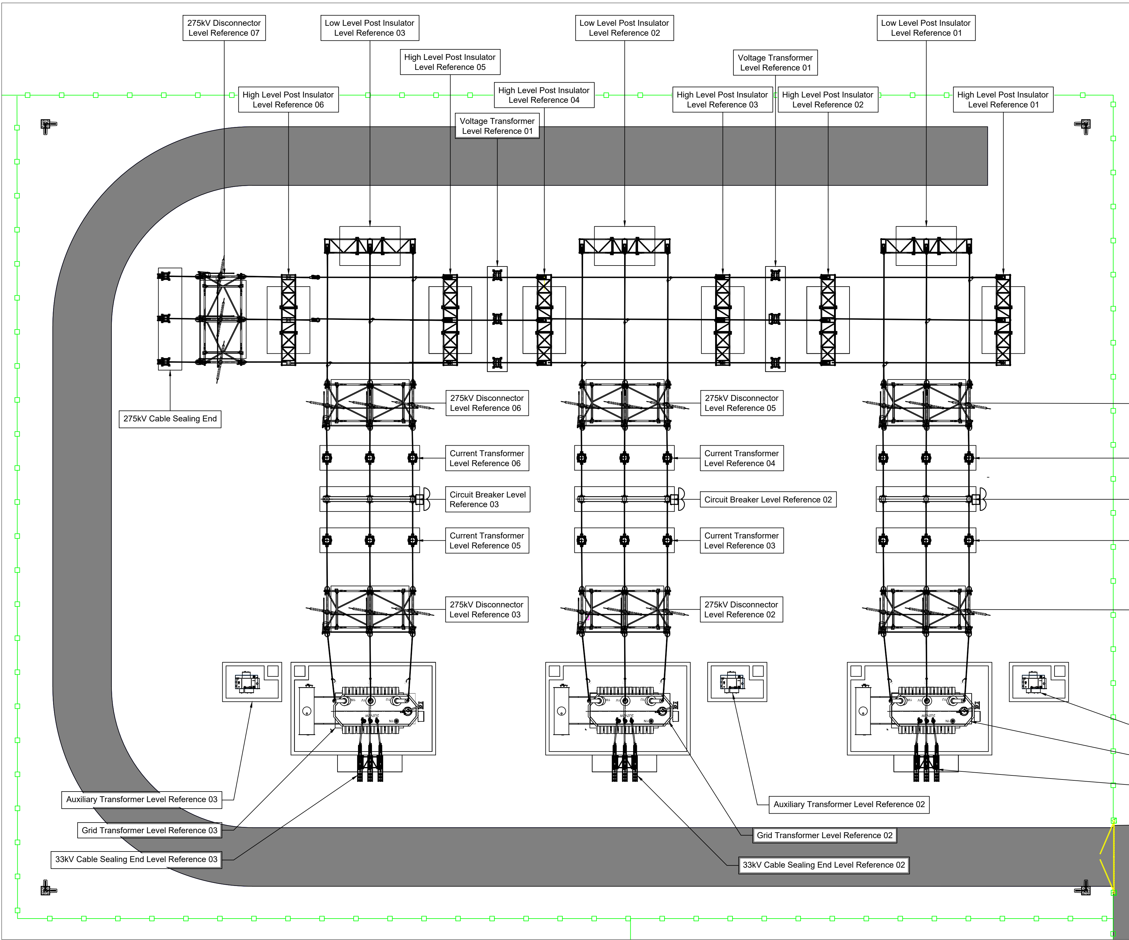
1 275kV Substation Structure Levels Plan Scale 1:200 @ A1
