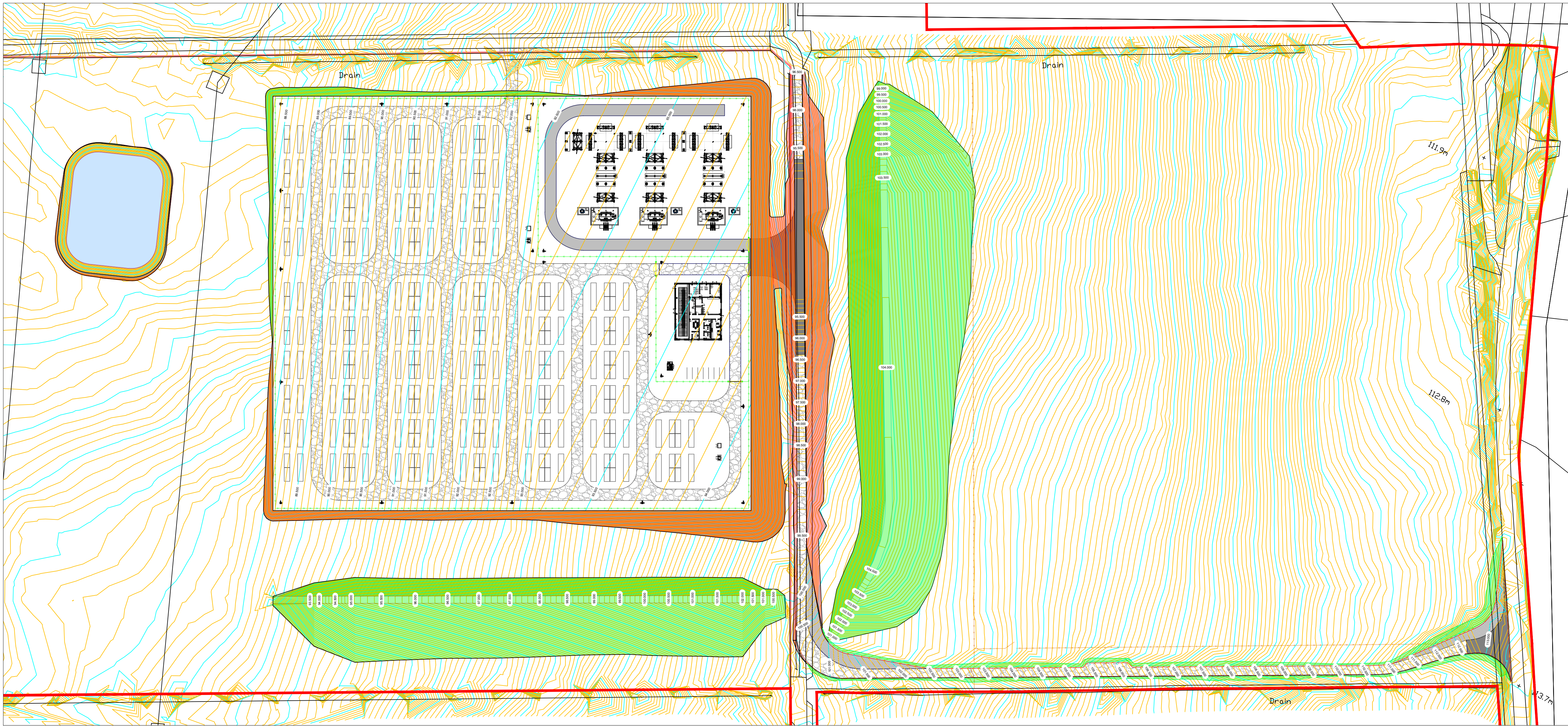
1 Site Finish Level Plan
